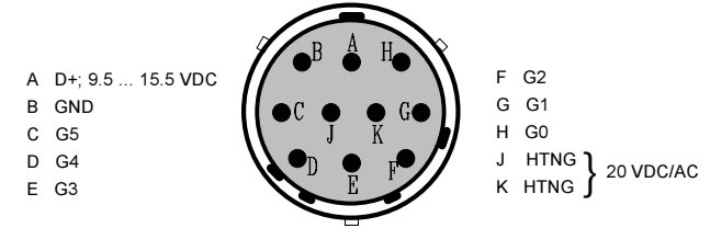
Figure 2. WAV151 connector
