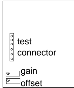
Figure 2.3 Calibration connector and potentiometers in the HMD 20/30UB/YB transmitters
